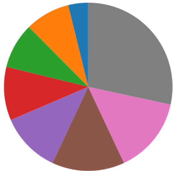
Sector Weights
